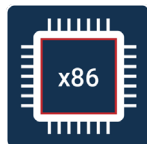
x86 Processor
